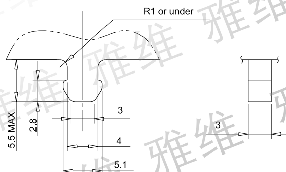
Striker shape (reference)
